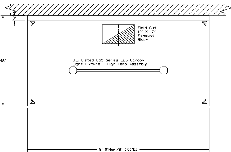
PLAN VIEW - Hood #2 (3C234) 8' 0.00" LONG 4824EX-2
